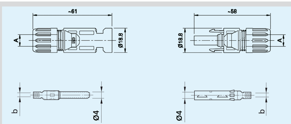
PV coupler plug PV-KST4 ...
